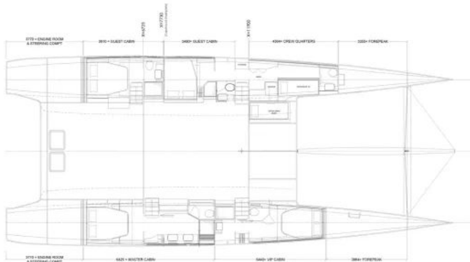
CABIN DECK LAYOUT
