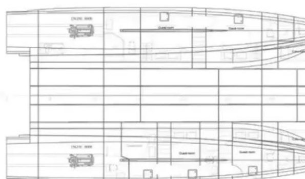
MAIN DECK
