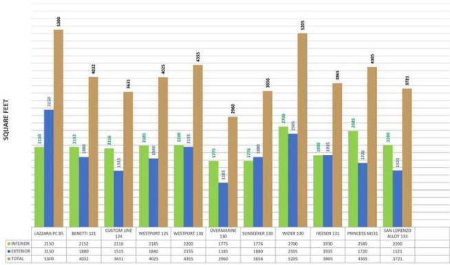
MARKET COMPARISON INT/EXT SQ FT: Lazzara Catamarans LPC 85' vs. 130' CLASS YACHTS (excludes crew and technical spaces)
