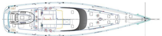
Lady K - Deck Plan
