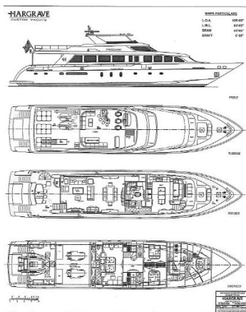
Hargrave Yacht Layout
