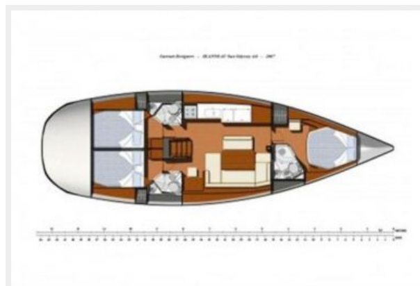
Manufacturer Provided Image: Layout Plan
