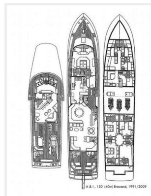
Layout
