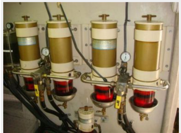
54' Sea Ray Racor fuel filters
