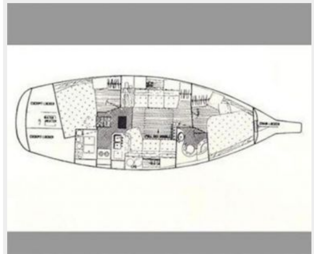
Layout drawing
