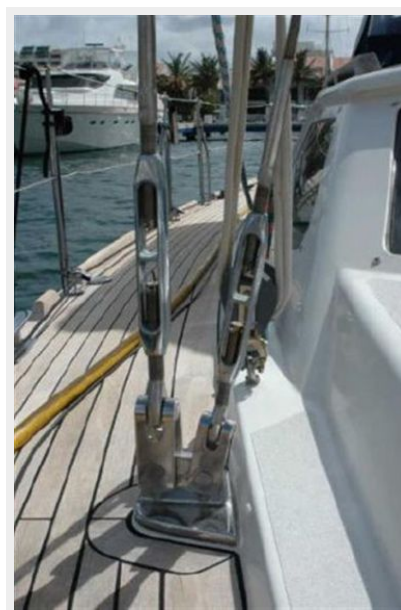
Shroud placement
