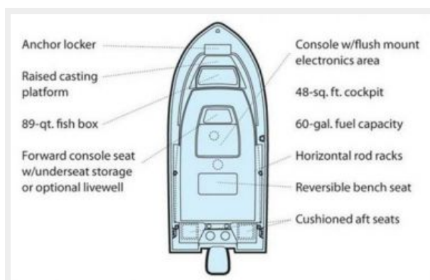
Layout
