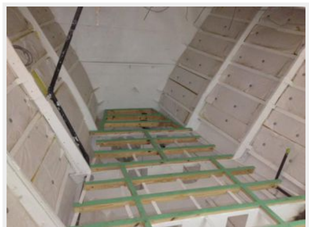
Floor Framing In Bow
