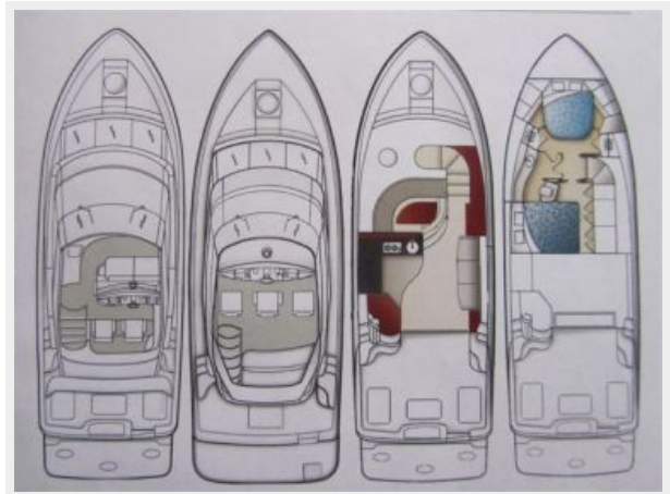
38' Carver layout
