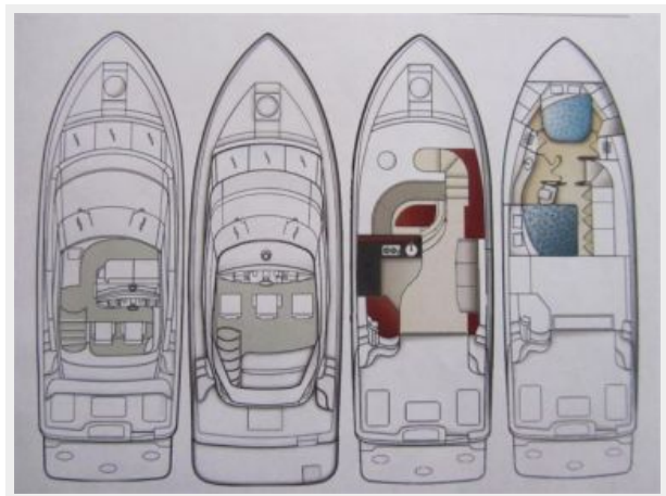
38' Carver layout
