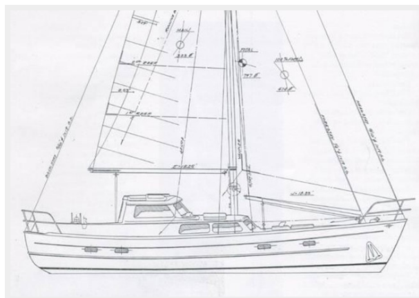
Profile Drawing - Sail Plan
