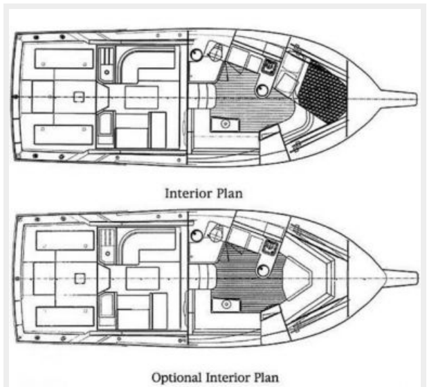
Floorplan
