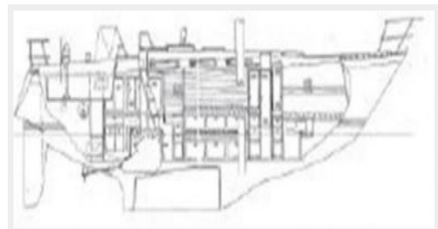
Stbd Profile Drawing
