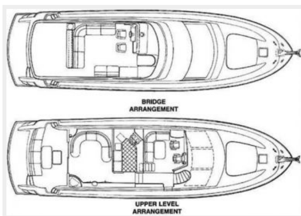
Flybridge & Main Deck Arrangements
