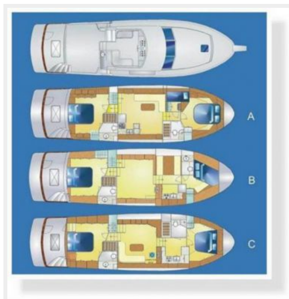
48' Novatec layout
