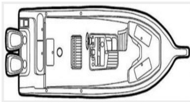
2600 - deck plan
