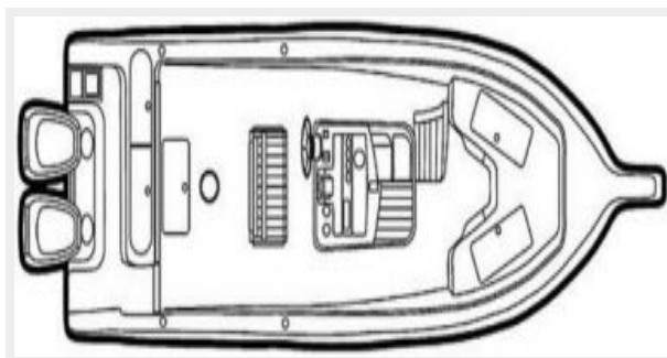
2600 - deck plan
