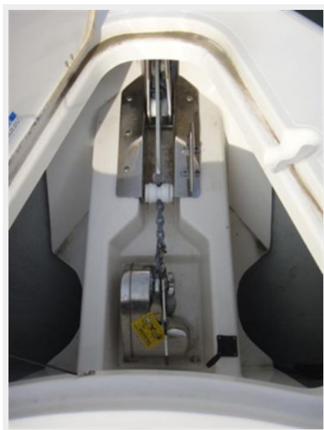
Anchor Windlass
