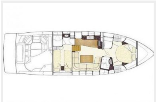
Layout Drawing
