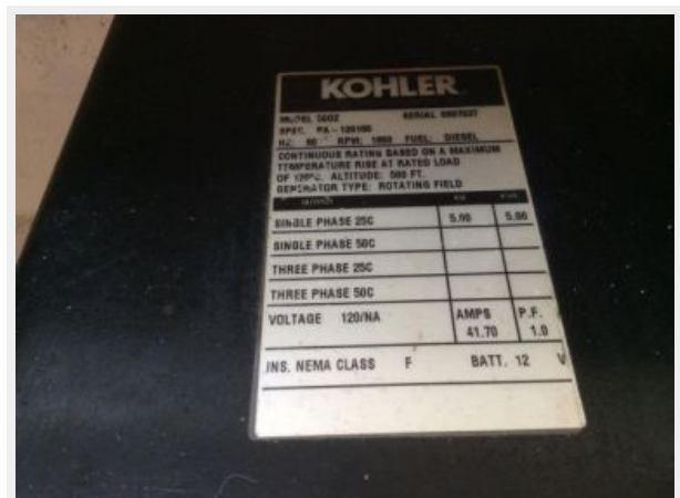
Generator specs
