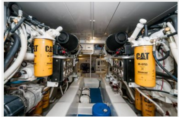
Engine Compartment
