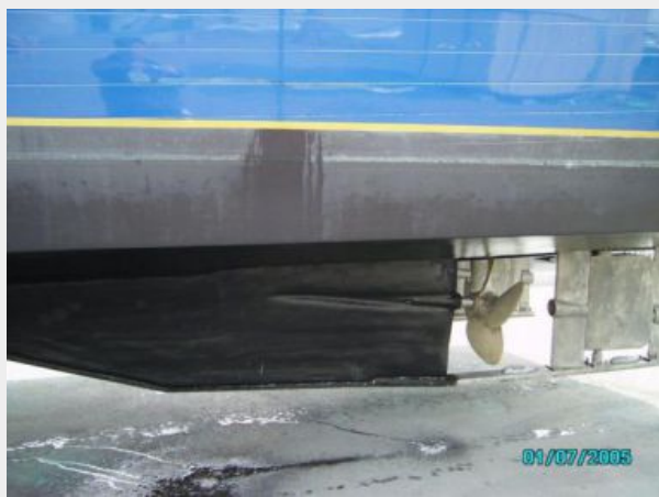
Shaft Protection
