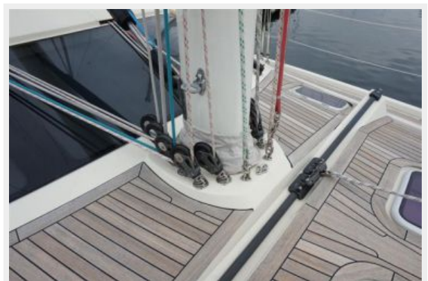
Mast Base
