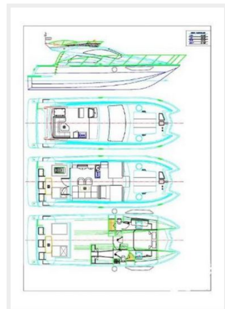
Mares 45 Flybridge - Layout
