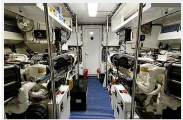
Engine room w walk through to guest or master
