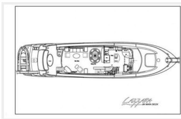
Main Deck
