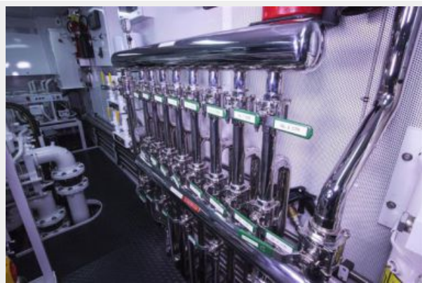
Fuel Manifold
