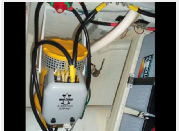
Thruster, Batteries & Charger
