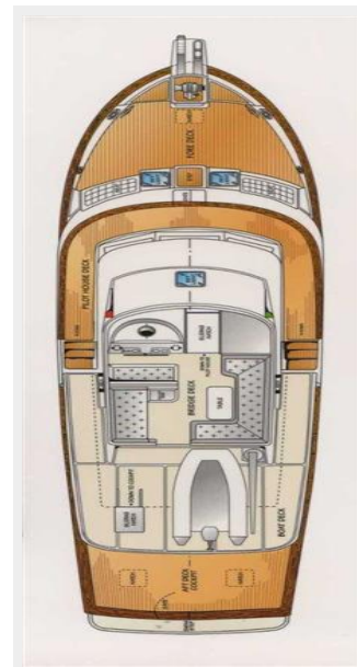
Layout Upper Deck
