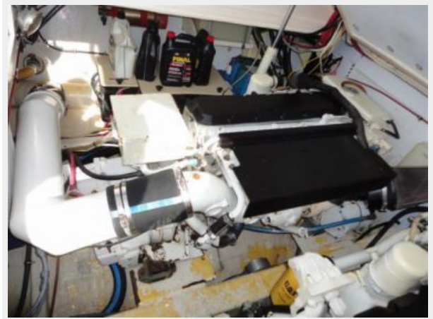
Inboard Side of Port Engine
