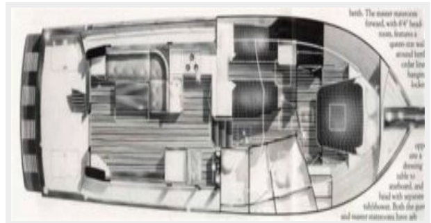
40' Cape Dory Layout
