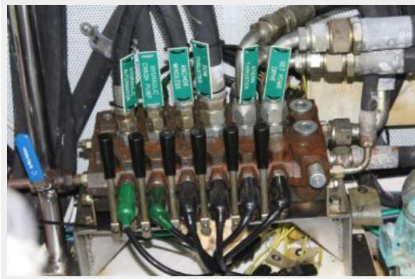
Hydraulic Manifold
