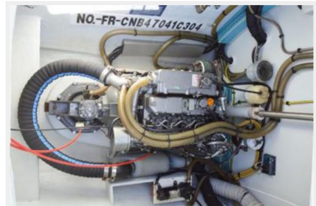
Starboard Engine
