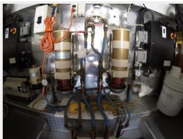
Engine Room
