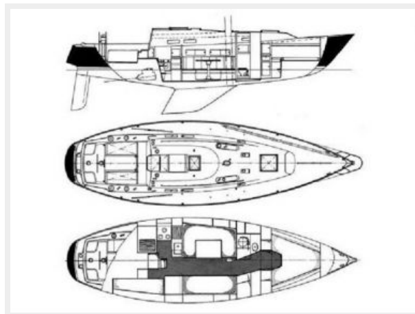
35' C&C layout2
