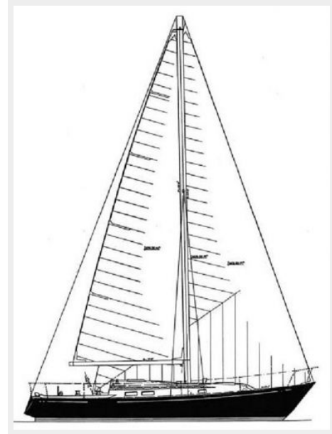
35' C&C Profile Layout1
