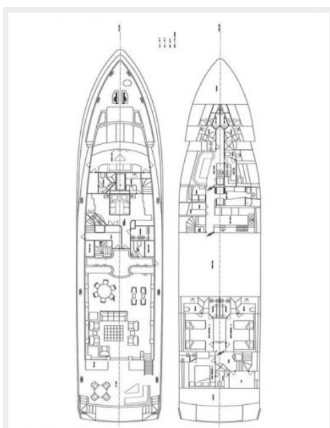
GA Plans
