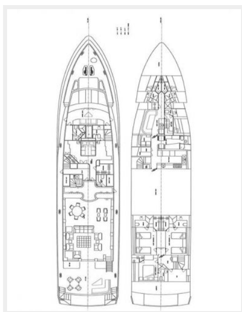
GA Plans
