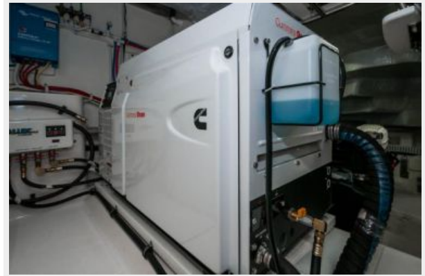
Generator
