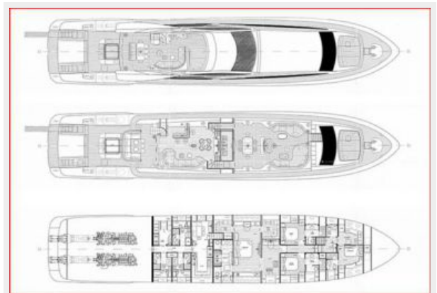
General Arrangement
