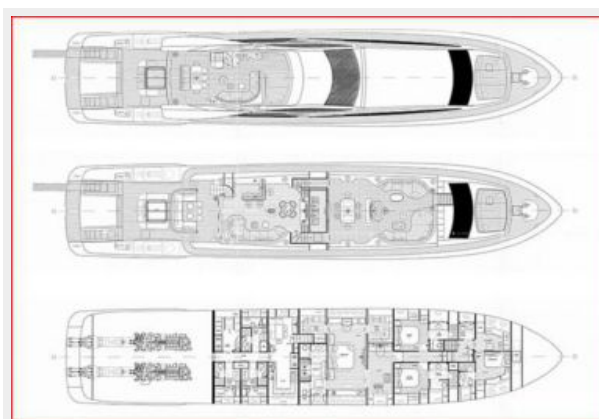
General Arrangement
