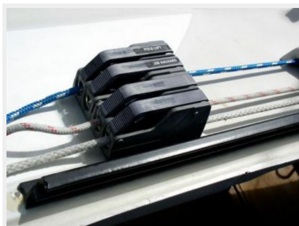
Halyard blocks. 2
