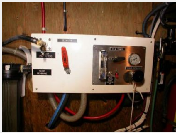
Watermaker - Forward machine room located under galley
