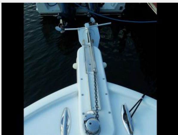
Windlass Detail
