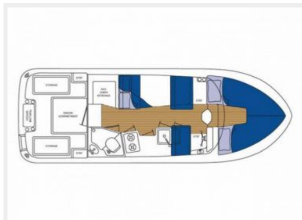
Blueprint Schematic
