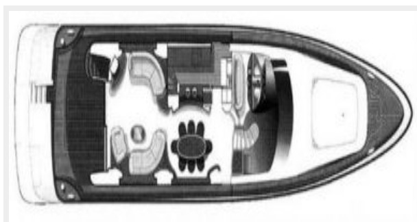
Upper floorplan
