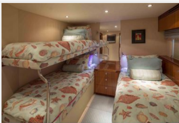
Port Stateroom
