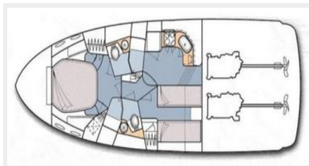
Stateroom Layout
