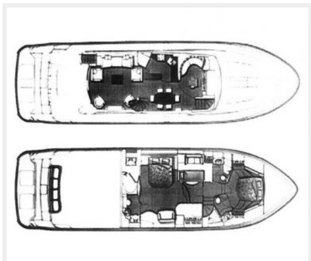
Main and Lower Deck Layout
